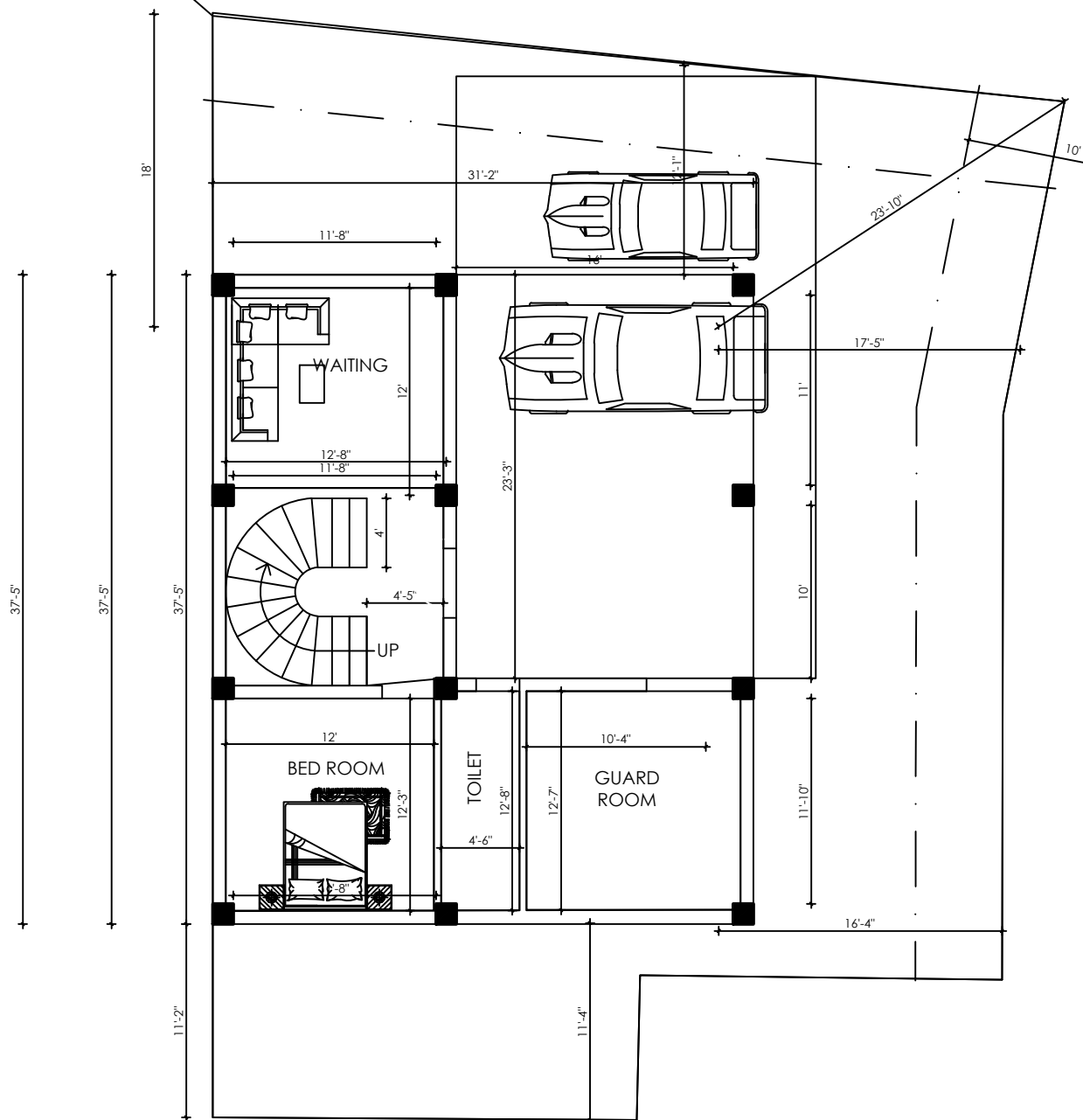
GROUND FLOOR PLAN AREA = 1100 SQ.FT TOTAL LAND AREA = 2900 SQ.FT
